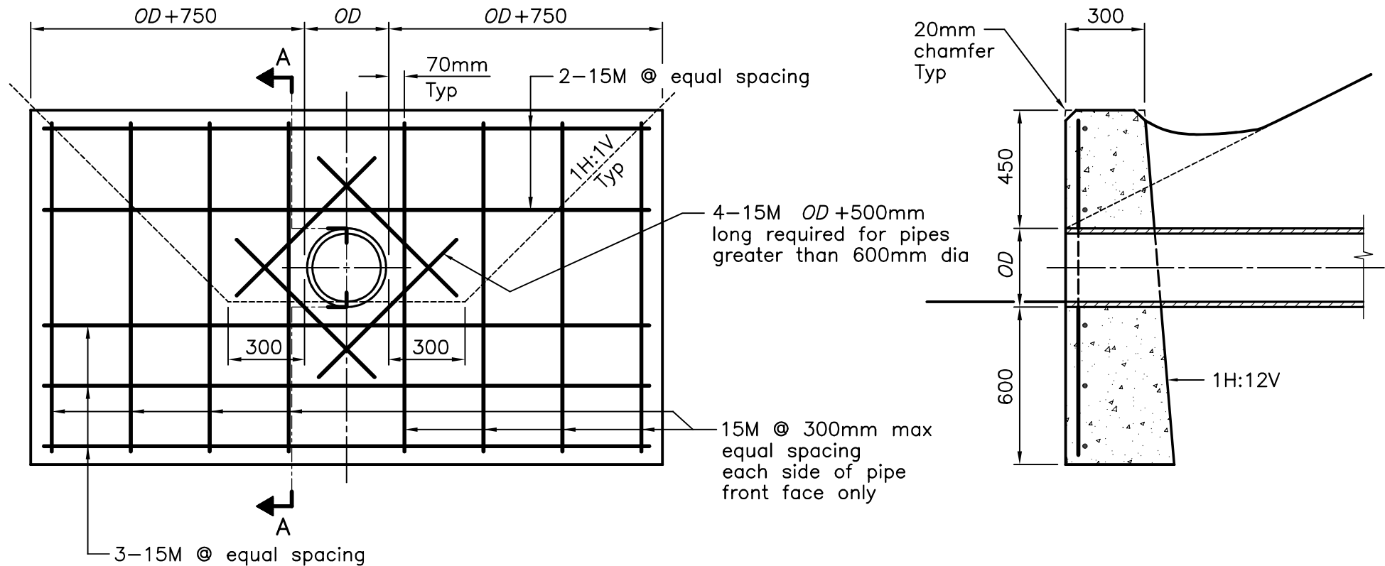
FRONT ELEVATION
